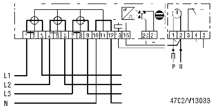
Figure 4. Connection diagram of the TE420Ns meter with floating double tariff control.
