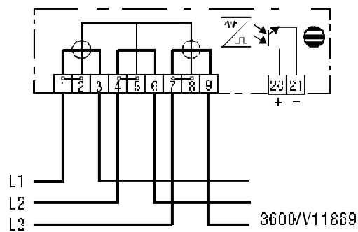
Figure 3. Connection diagram of the E420s meter.
