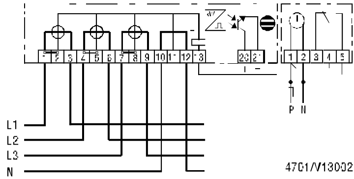
Figure 1. Connection diagram of the TE420Ns meter with tariff control.
