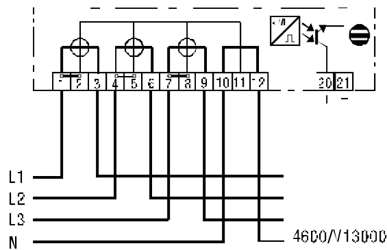
Figure 2. Connection diagram of the E420Ns meter
